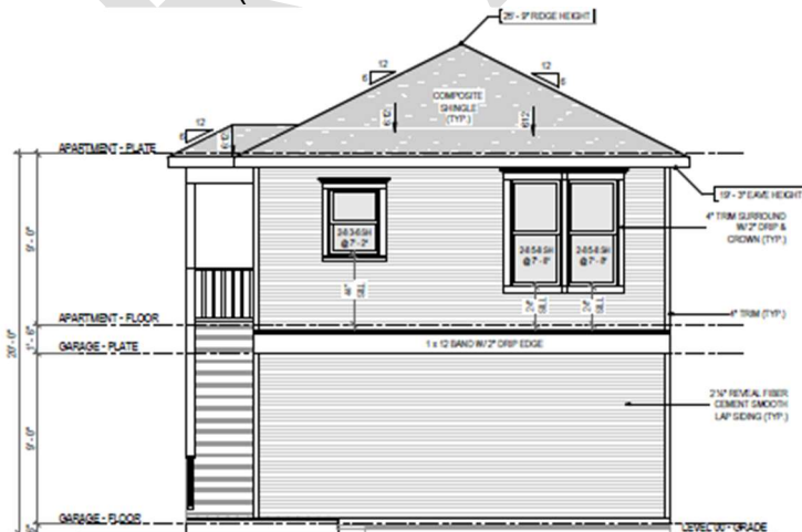
PROPOSED SOUTH GARAGE ELEVATION
