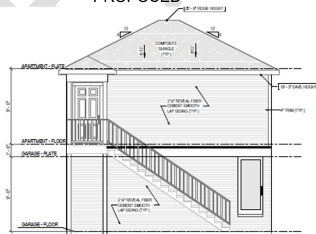
PROPOSED WEST GARAGE ELEVATION
