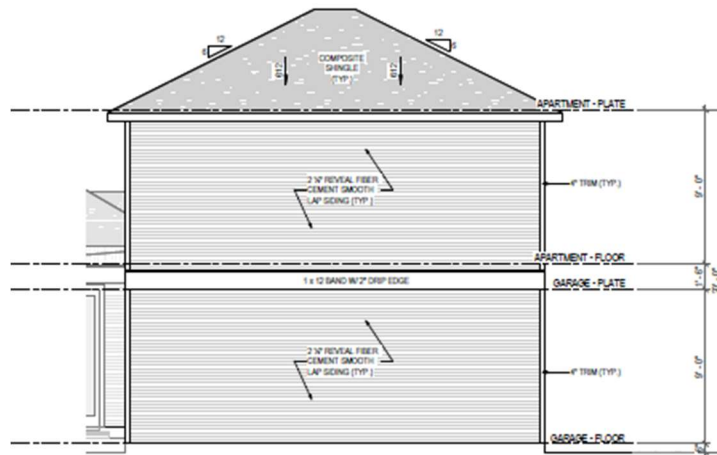
PROPOSED EAST GARAGE ELEVATION
