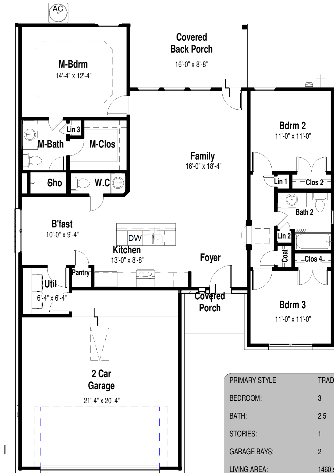
1 Floor Plan Brochure 1/8" = 1'-0"
