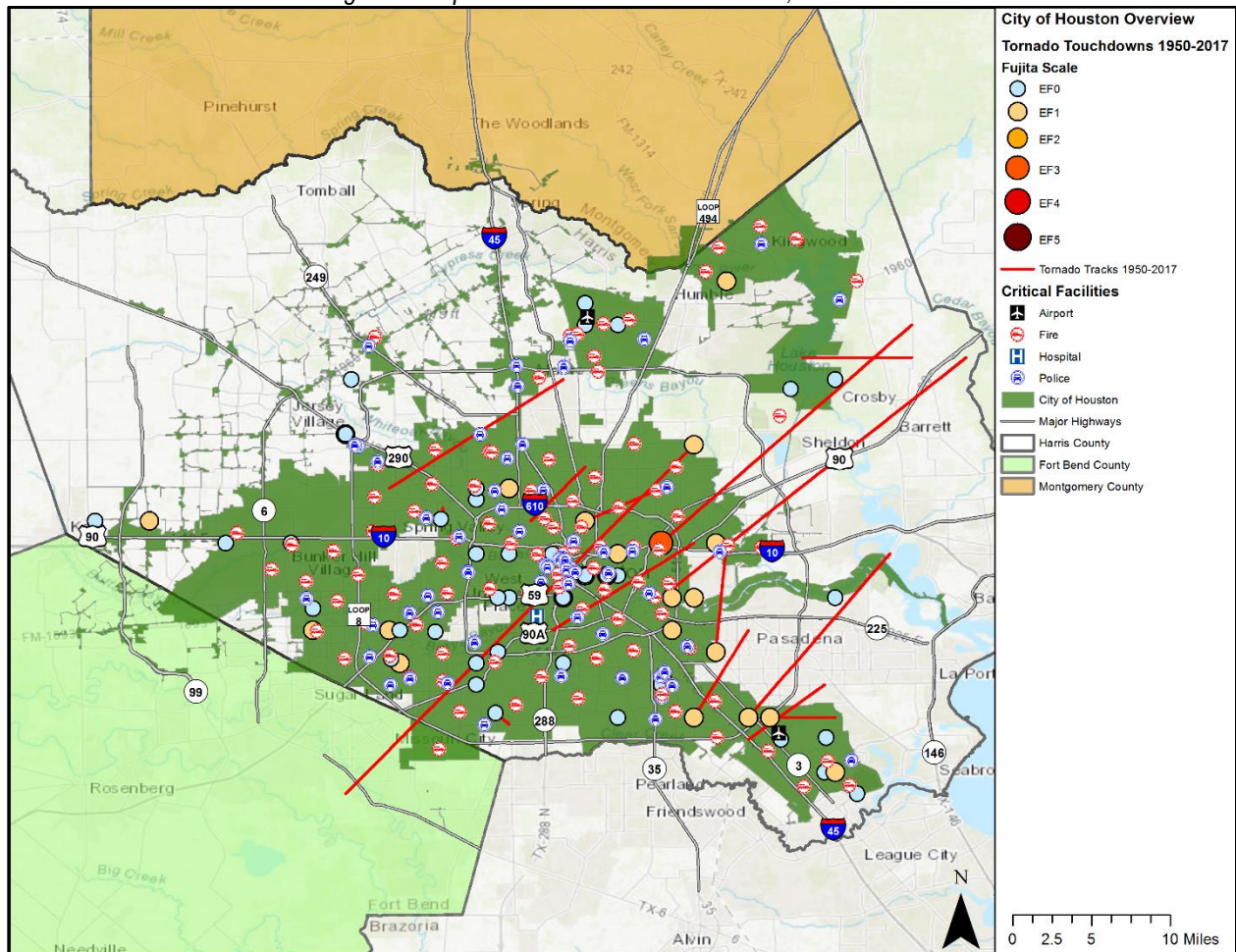
Figure 12: Spatial Historical Tornado Events, 1950-2017
