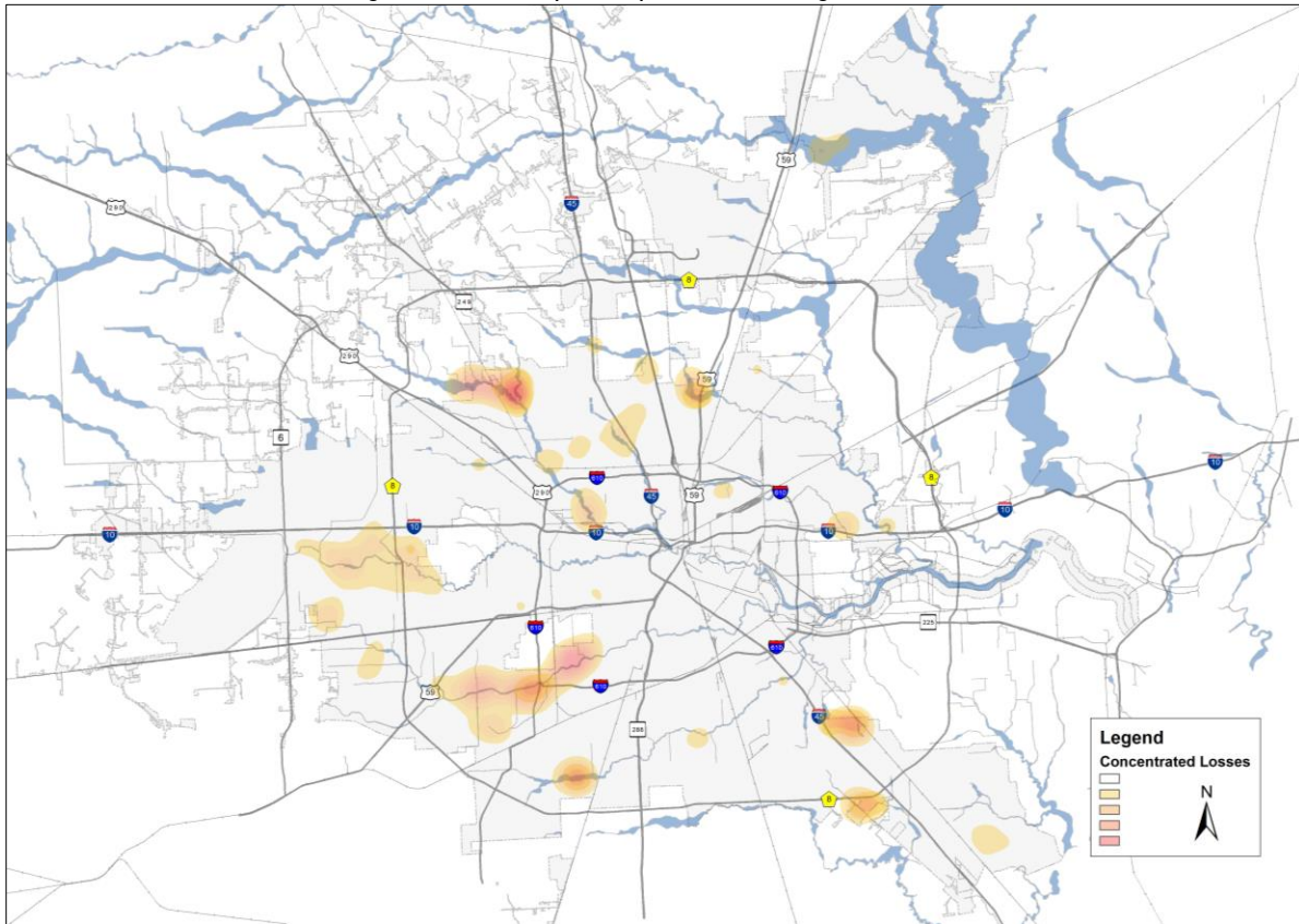
Figure 9: Heat Map of Repetitive Flooding in Houston
